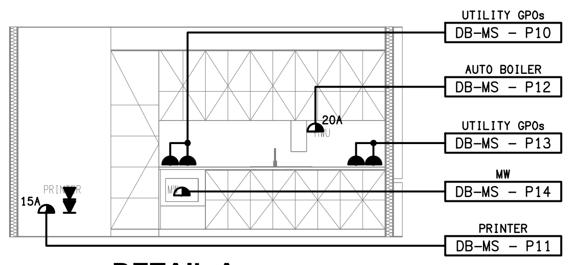
DETAIL A KITCHENETTE ELEVATION SCALE 1:50
