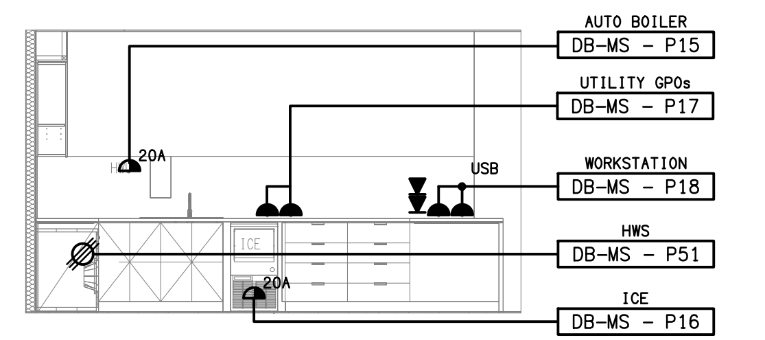
DETAIL B UTILITIES BENCH ELEVATION 1 SCALE 1:50
