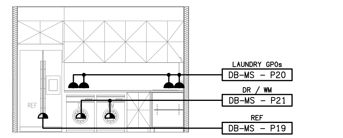
DETAIL C UTILITIES BENCH ELEVATION 2 SCALE 1:50
